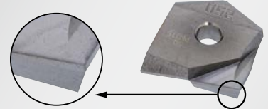
刃先部拡大 Magnified view of cutting edge
